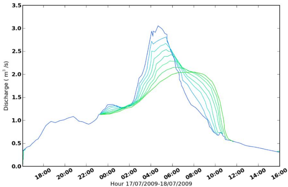
Figure 5: Pond Network Model output for July 2009 for a 1 in 100 year rainfall event. Simulation of 30 hypothetical RAFs of 550\text{m}^3 storage each. Scenario shows a 30% reduction in peak flow.
