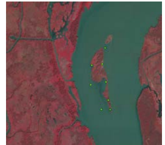
Figure 1. The Atchafalaya River Island had grown to 90 acres as of Dec 2009.
